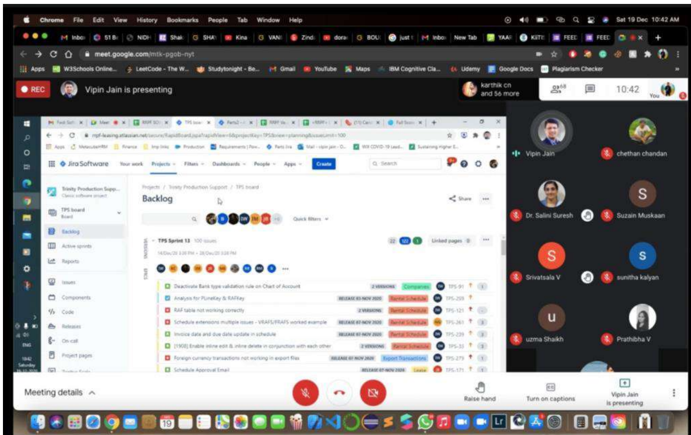
Photo 3 : BacklogDemo Testcase
